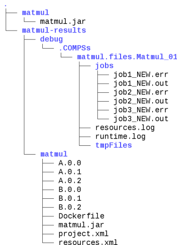
Figure 14: Result and log folders of a Matmul execution with COMPSs and Docker
